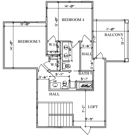
2ND FLOOR PLAN NOT TO SCALE
