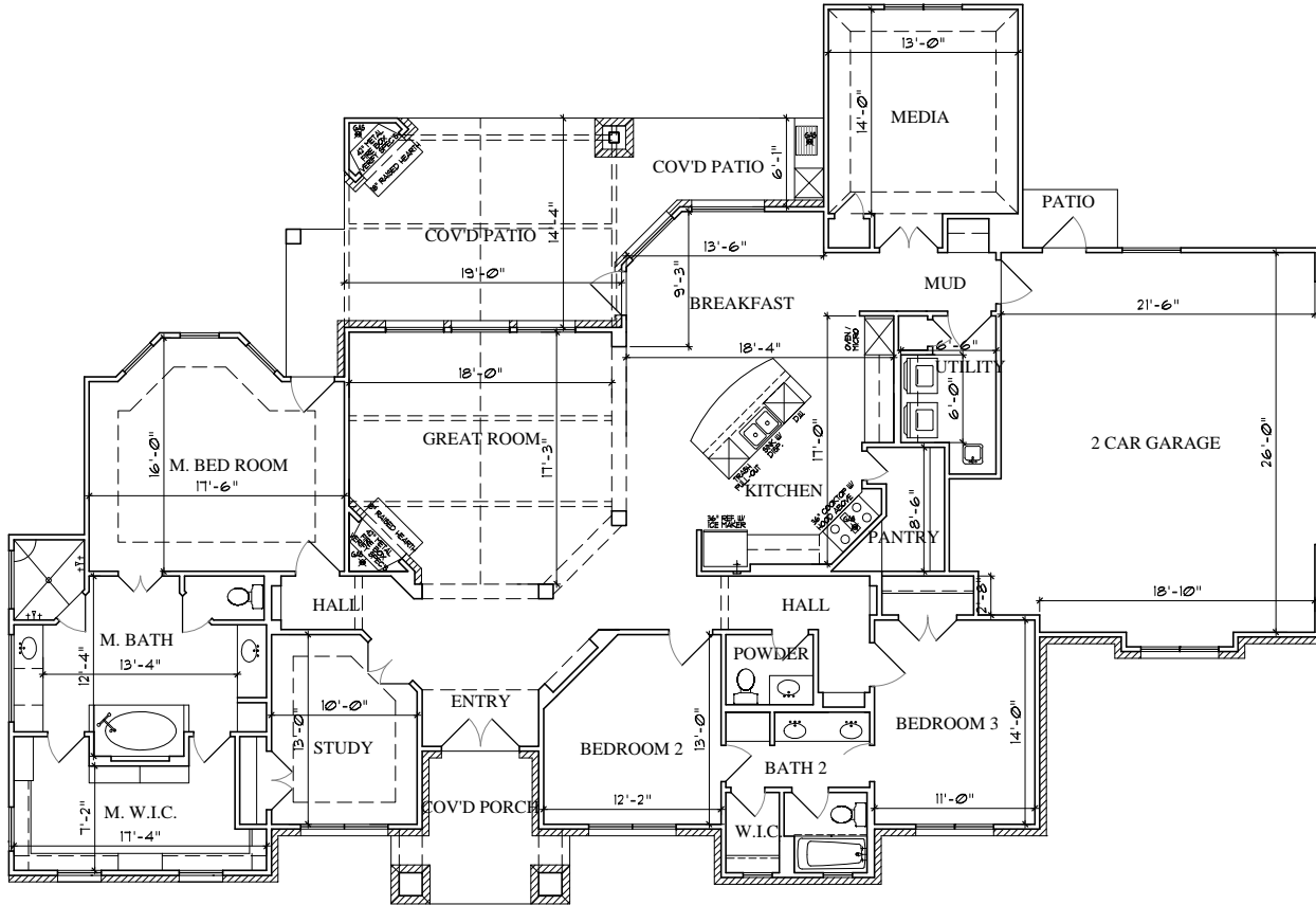
FLOOR PLAN NOT TO SCALE
