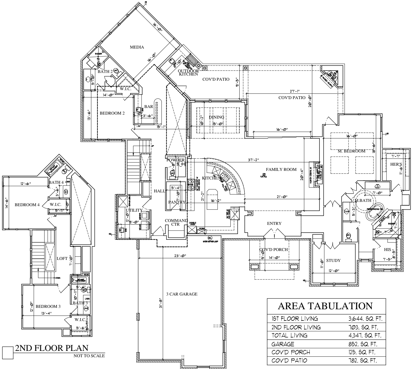
1ST FLOOR PLAN NOT TO SCALE
